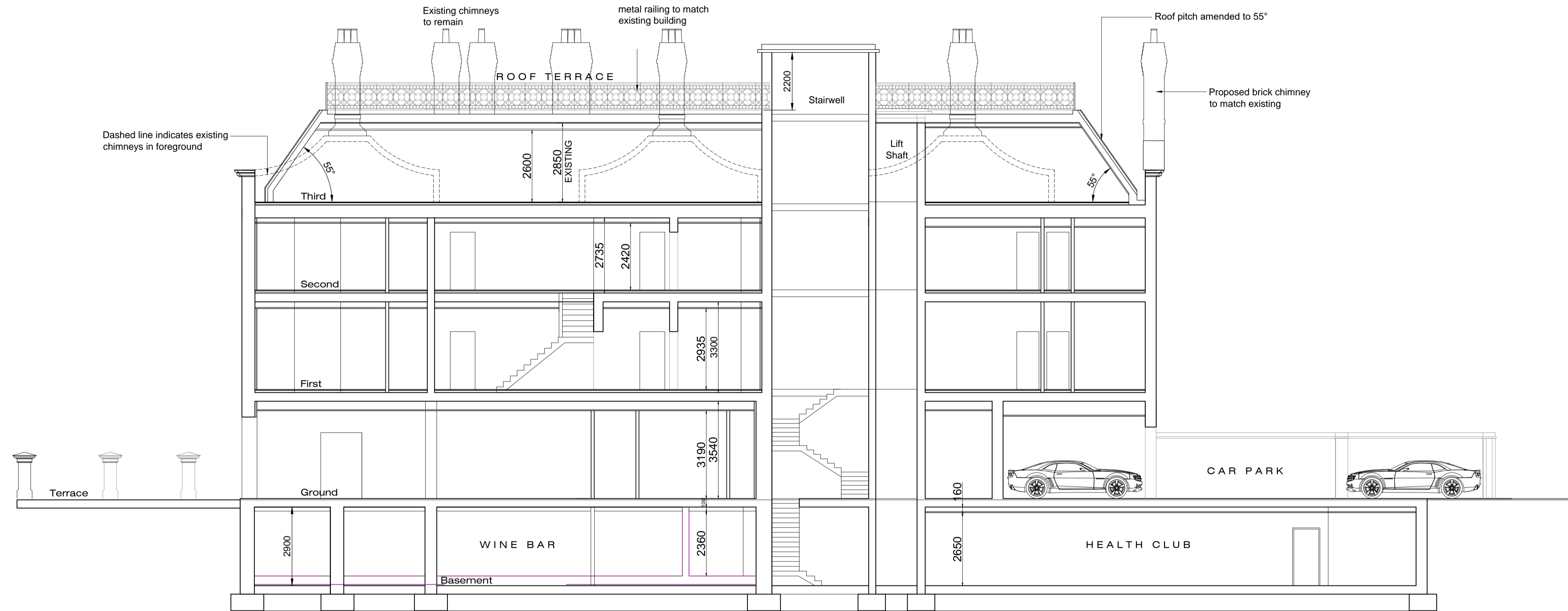
PLANNING SECTION A-A Scale 1:100
